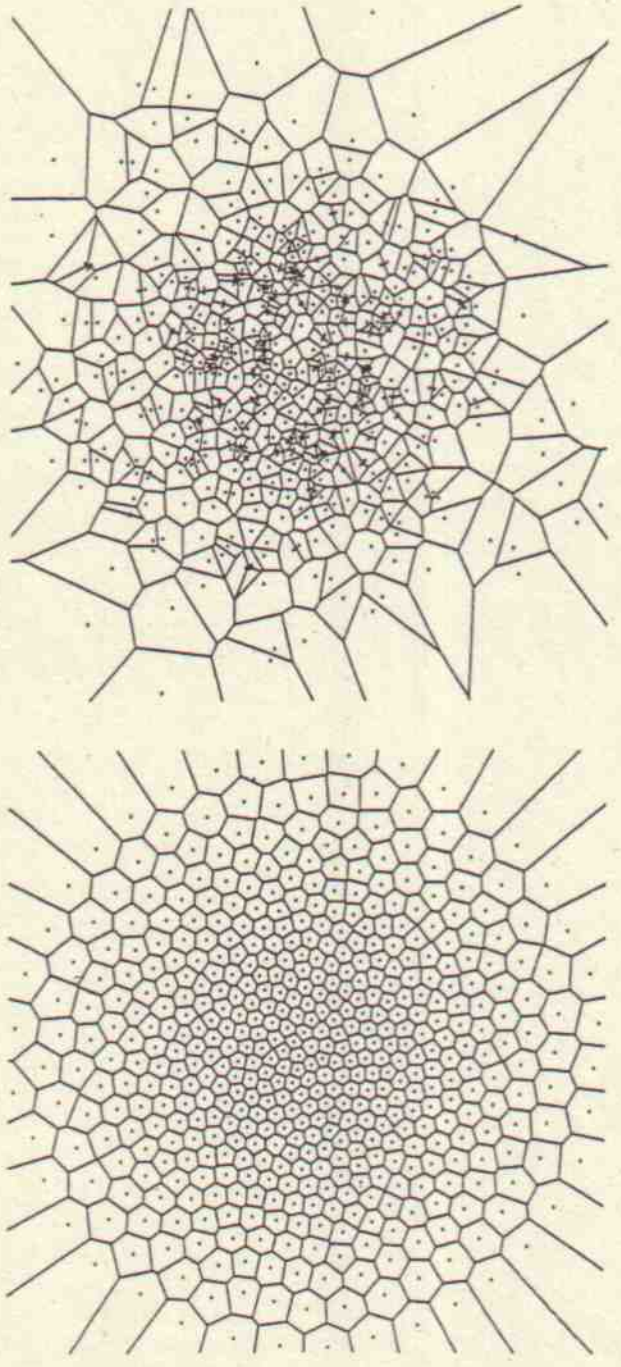
Fig. 2. Two N -quantizers (and their Voronoi diagram) related to bi-variate normal distribution N(0; I_2) ( N = 500 ); which one is the best?
